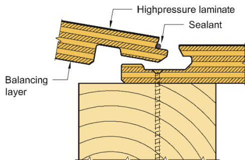
Fig. 2 Mounting principle for BerryAlloc Wall&Water.
