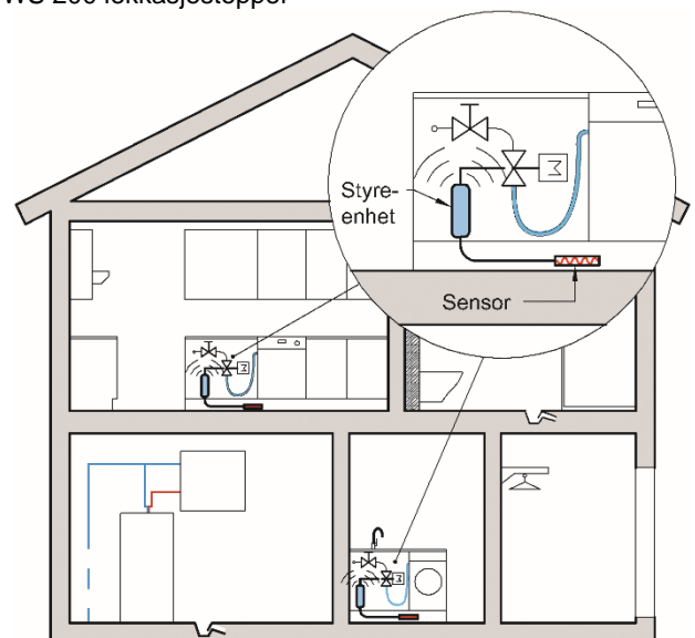
Fig. 2 Systemskisse for WaterStop WS 50 lekkasjestopper
