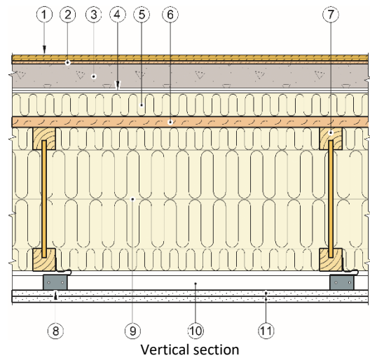
Fig. 11 Principle design of bathroom ground floor. Joist size and spacing according to specific structural calculations. In floors between modules are wind barrier and ceiling board replaced by steel mesh
