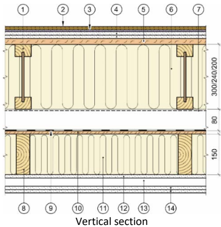
Fig. 9 Principle design of standard separating floors between modules. Upper part is the floor structure of the upper module and lower part is the ceiling structure of the lower module. Joist size and spacing according to specific structural calculations
