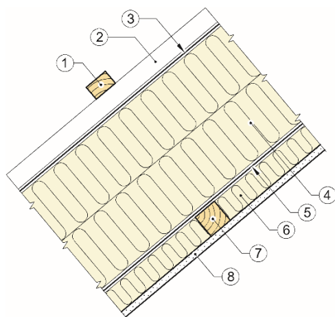
Fig. 13 Principle design of flat roof construction. Joist size and spacing according to specific structural calculations
