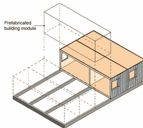
Fig. 1 Principle use of Unihouse building modules.
