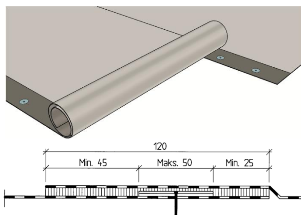
Fig. 1 Polar 5000 is mechanically fastened with 120 mm welded overlap joint
