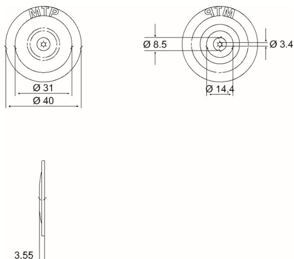
Fig. 6 Milletech Itech 40 steel washer for use together with wood screws
