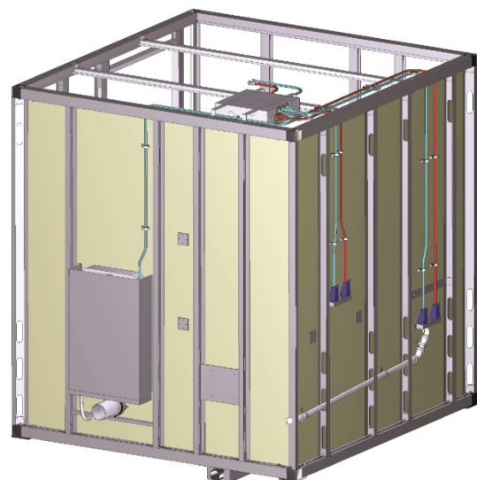
External view; Bathsystem Superlight Bathroom Pod
